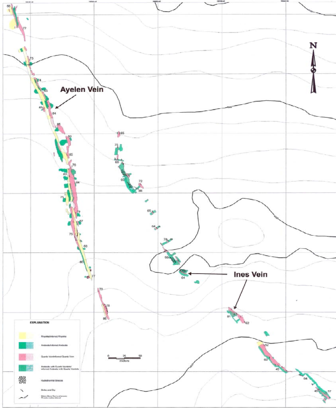
Figure 9-3: Geologic Plan Map of Ayelén and Inés Veins (Excerpted from Figure 6, Blanchflower 2007)
