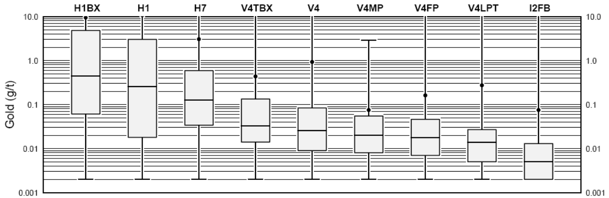
Figure 17-1: Au Box Plot For Select Lithologic Units
