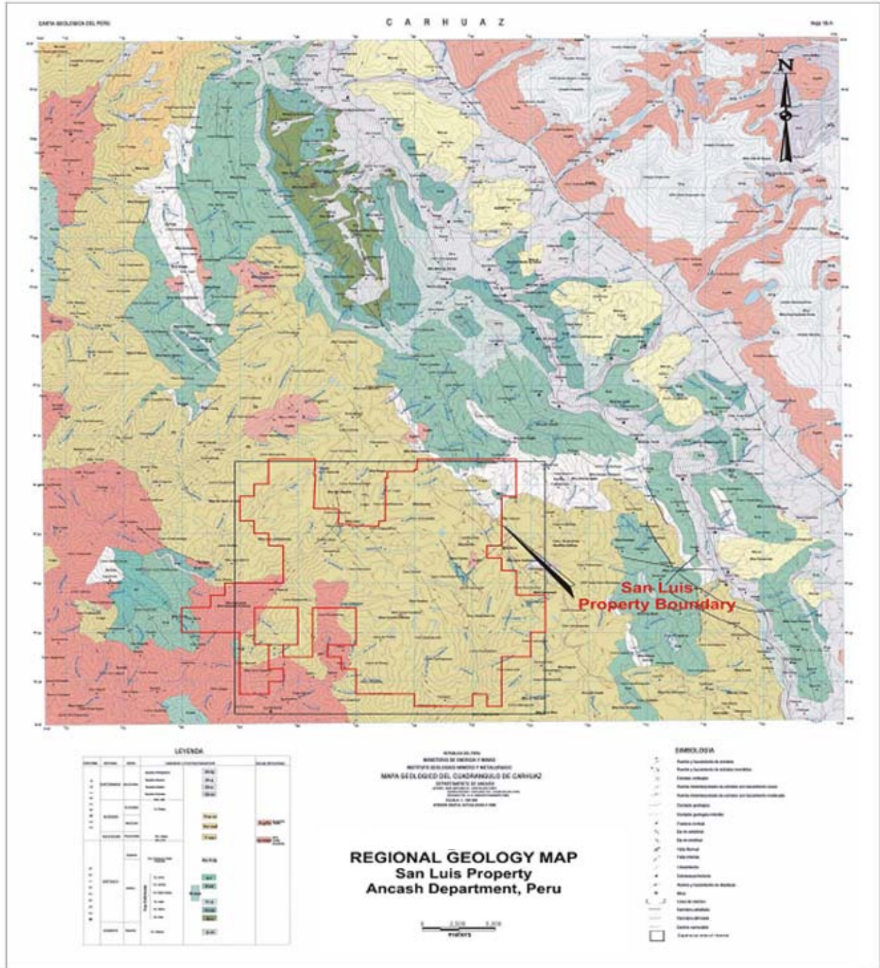
Figure 7-1: Regional Geology (Excerpted from Figure 4, Blanchflower 2007)
