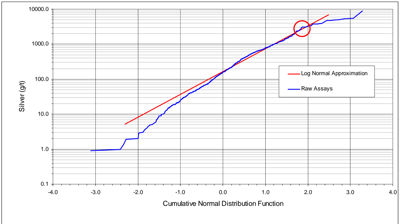
Figure 17-4: Ayelén Ag Cumulative Probability Plot
