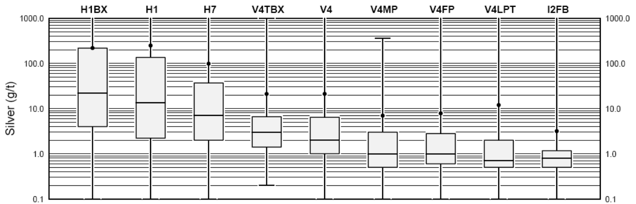
Figure 17-2: Ag Box Plot For Select Lithologic Units
