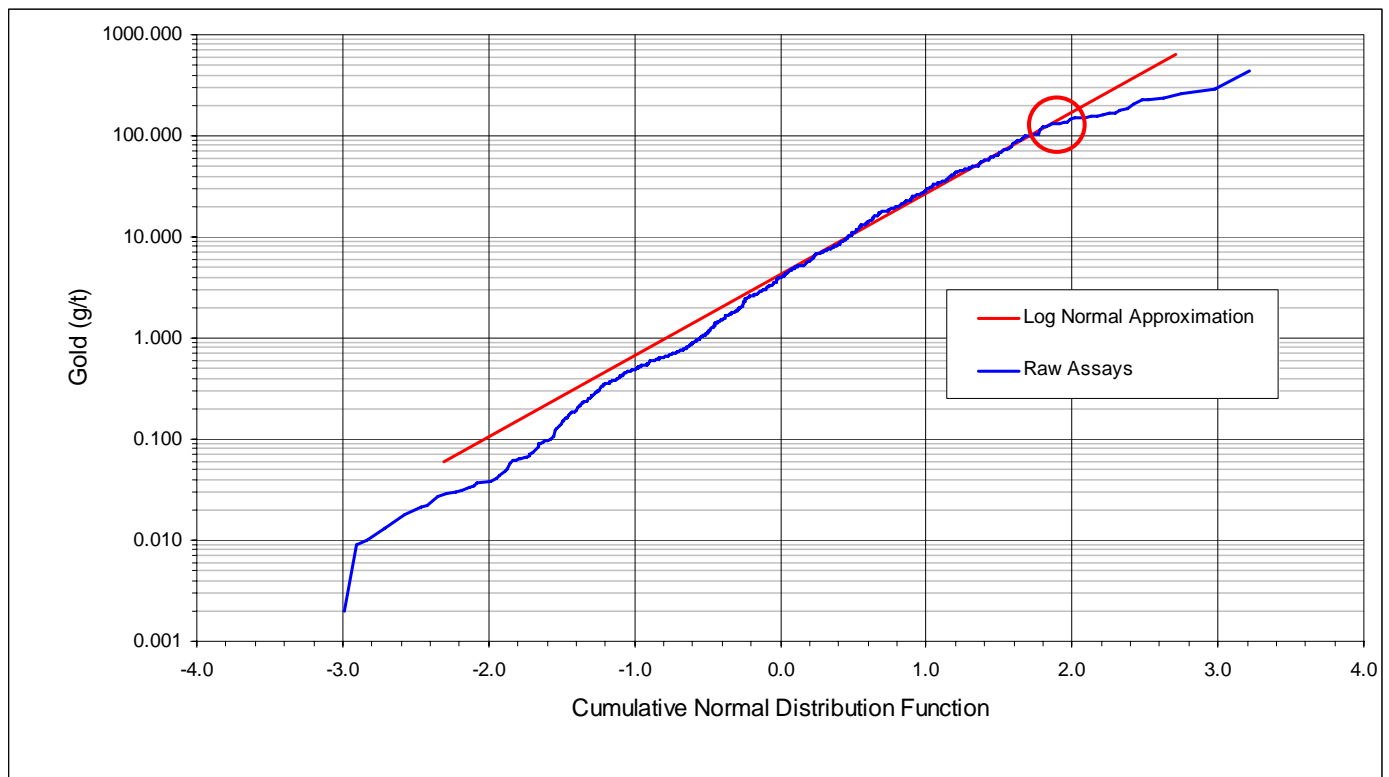
Figure 17-3: Ayelén Au Cumulative Probability Plot
