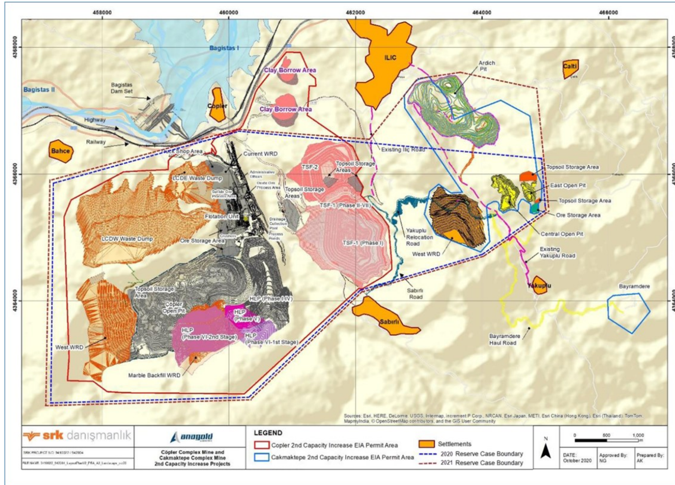
Figure 13.8 CDMP21TRS Reserve Case Site Plan
