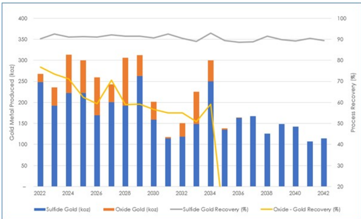
Figure 1.11 CDMP21TRS Reserve Case Gold Production
