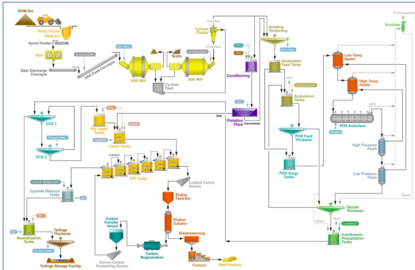
Figure 14.4 Process Flow Sheet for Sulfide Plant
