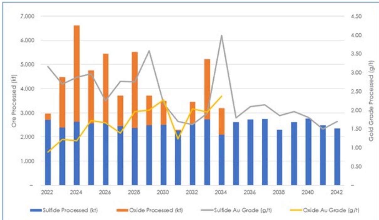
Figure 19.2 CDMP21TRS Reserve Case Processing
