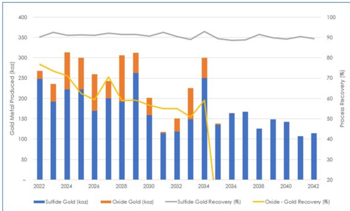
Figure 13.11 CDMP21TRS Reserve Case Gold Production and Recovery
