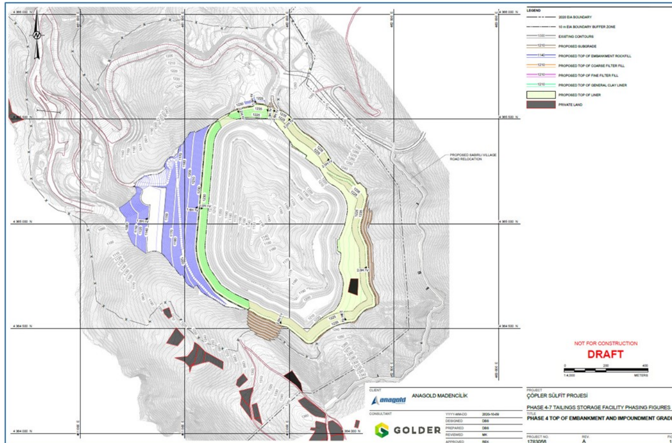
Figure 15.3 Phase 4 – Top of Embankment and Impoundment Grade
