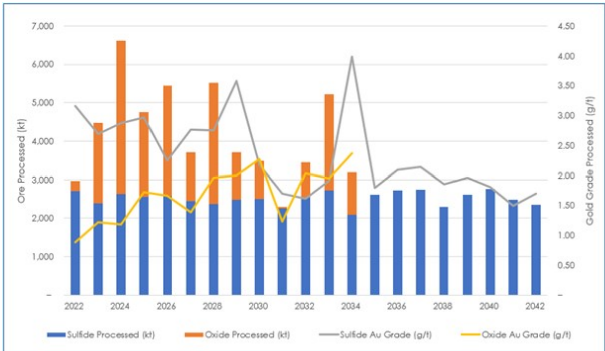
Figure 1.10 CDMP21TRS Reserve Case Processing
